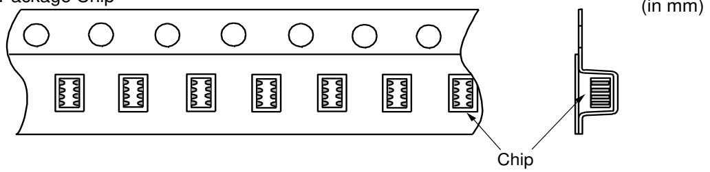
Fig.2 Dimension of Reel
