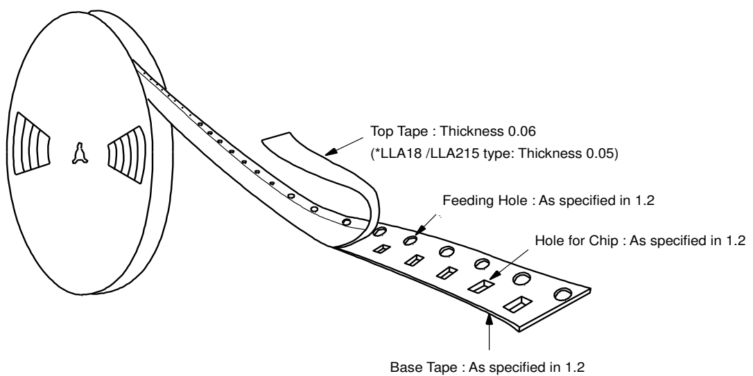
Fig3 Taping Diagram
