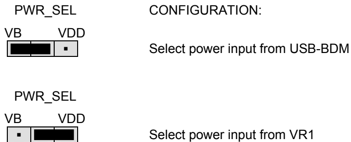
Figure 1: PWR_SEL Option Header
