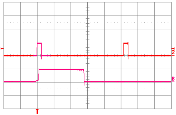
Fig. 1.5V.18: Load current (top trace, 20 \text{ A}/\text{div} ., 20 \text{ ms}/\text{div} .) into a 10 \text{ m}\Omega short circuit during restart, at V_{in} = 24\text{V} . Bottom trace ( 20 \text{ A}/\text{div} ., 2 \text{ ms}/\text{div} .) is an expansion of the on-time portion of the top trace.
