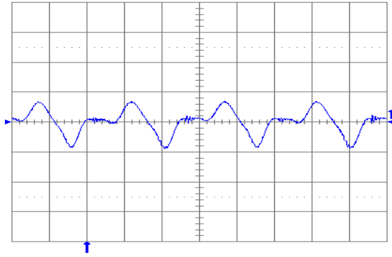
Fig. 1.5V.13: Output voltage ripple (20 mV/div.) at full rated load current into a resistive load with C_o = 10 \mu\text{F} tantalum + 1\mu\text{F} ceramic and V_{in} = 24\text{V} . Time scale: 1 \mu\text{s}/\text{div} .
