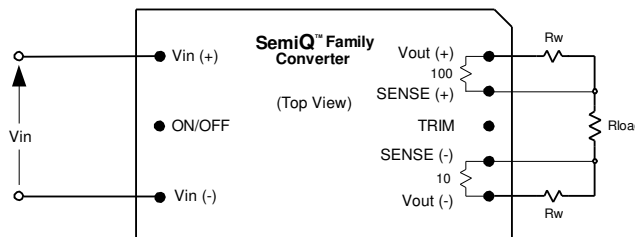
Figure B. Remote sense circuit configuration.
