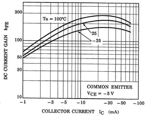
Fig. 10.16 RN2904 h_{FE-IC}
