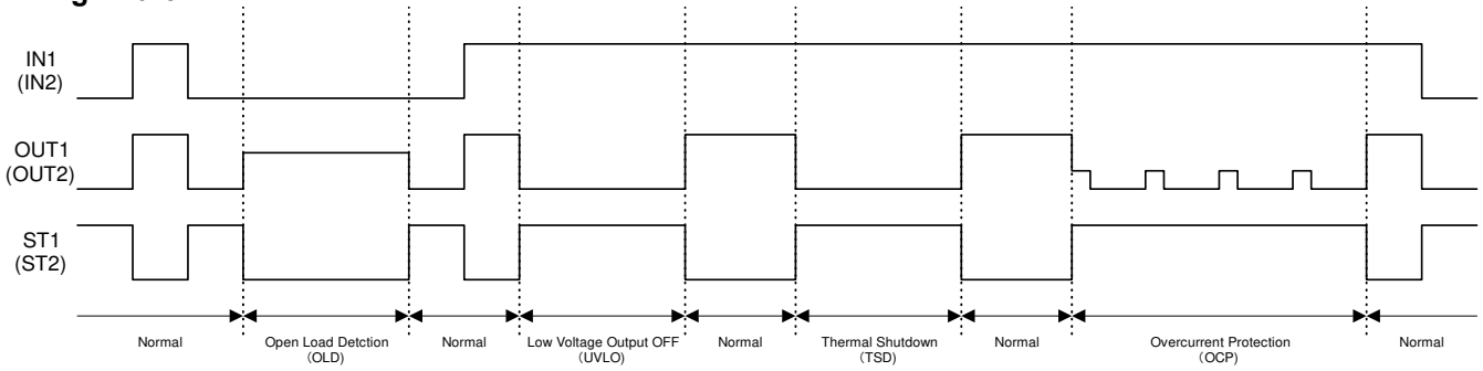
Figure 43. Timing Chart
