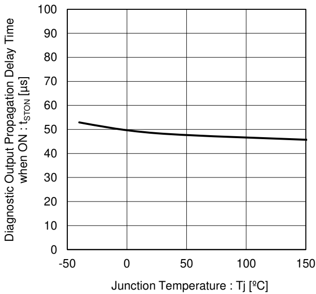
Figure 25. Diagnostic Output Propagation Delay Time when ON vs Junction Temperature
