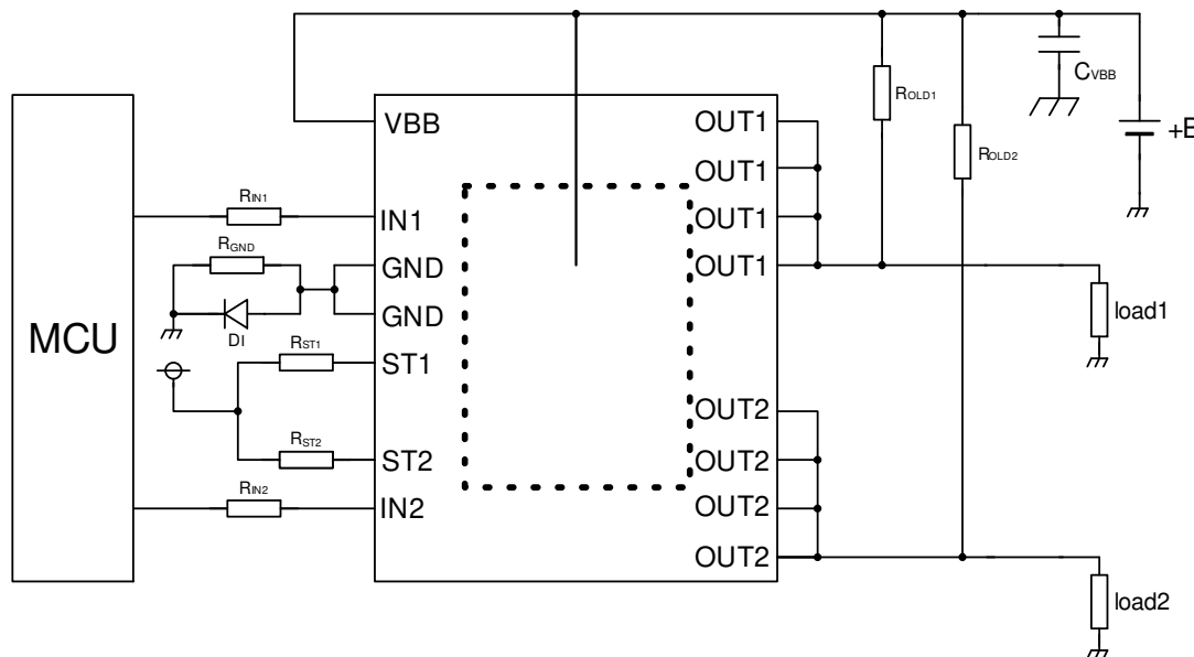
Figure 1. Application Circuit
