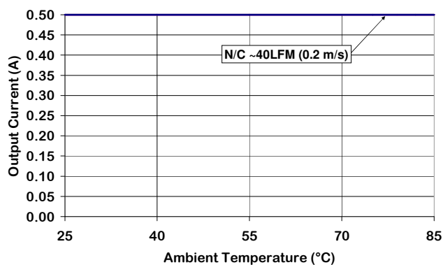
Figure 4. Output Current Derating vs Ambient Temperature & Airflow (Open Frame module) Airflow from pin 1 to 2; Vin = 12V
