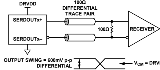
Figure 72. DC-Coupled Digital Output Termination Example
