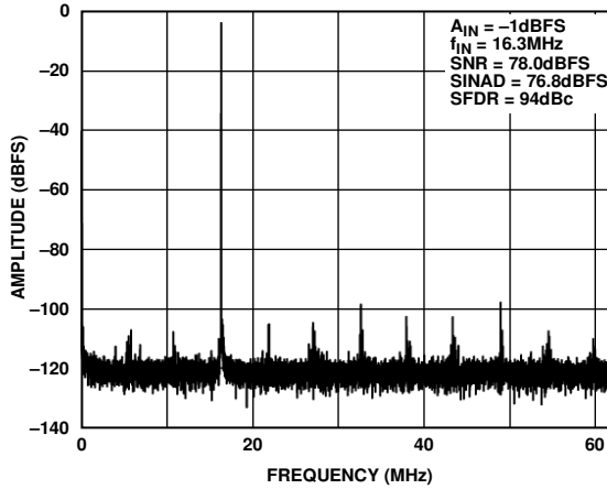
Figure 22. Single-Tone 32k FFT with f_{IN} = 16.3\text{ MHz} , f_{SAMPLE} = 125\text{ MSPS} , V_{REF} = 1.0\text{ V}
