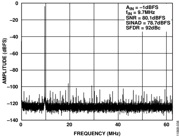
Figure 5. Single-Tone 32k FFT with f_{IN} = 9.7 MHz , f_{SAMPLE} = 125 MSPS , V_{REF} = 1.4 V
