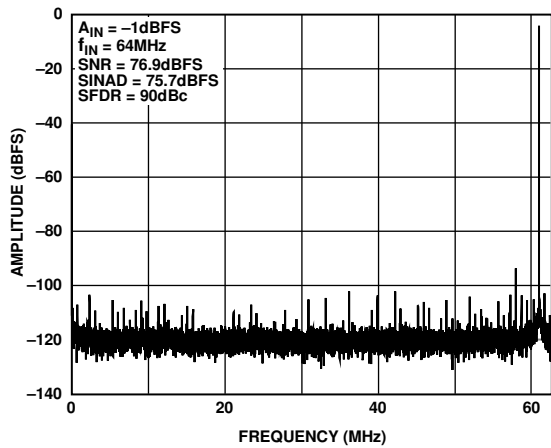
Figure 23. Single-Tone 32k FFT with f_{IN} = 64\text{ MHz} , f_{SAMPLE} = 125\text{ MSPS} , V_{REF} = 1.0\text{ V}
