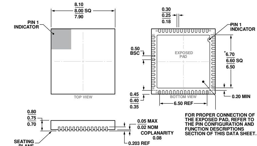
Figure 75. 56-Lead Lead Frame Chip Scale Package [LFCSP_WQ] 8 mm x 8 mm Body, Very Very Thin Quad (CP-56-9) Dimensions shown in millimeters
