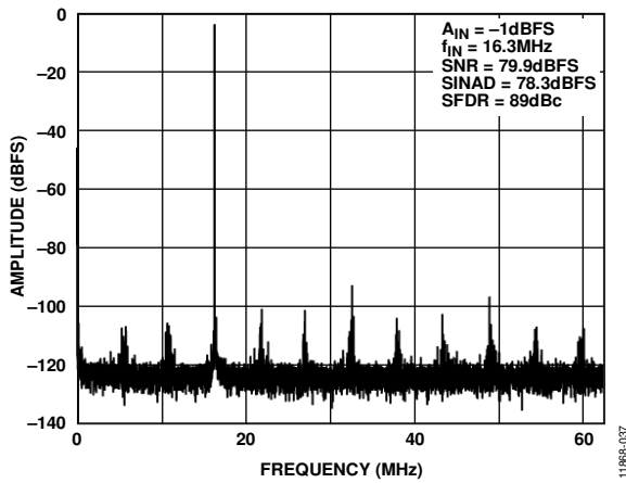
Figure 6. Single-Tone 32k FFT with f_{IN} = 16.3 MHz , f_{SAMPLE} = 125 MSPS , V_{REF} = 1.4 V
