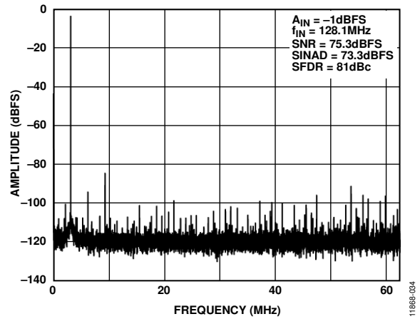
Figure 8. Single-Tone 32k FFT with f_{IN} = 128.1 MHz , f_{SAMPLE} = 125 MSPS , V_{REF} = 1.4 V
