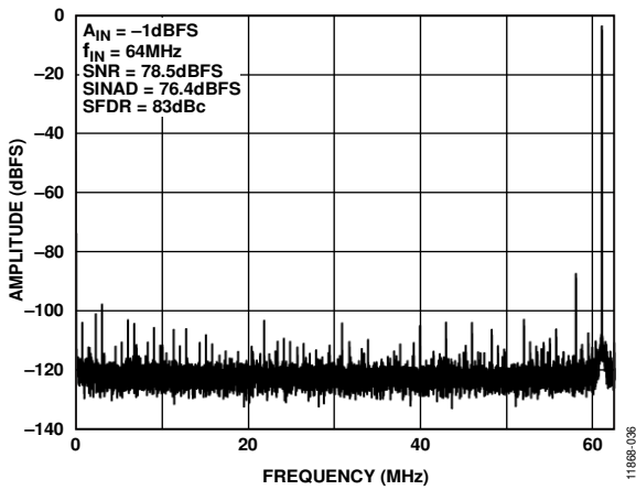
Figure 7. Single-Tone 32k FFT with f_{IN} = 64 MHz , f_{SAMPLE} = 125 MSPS , V_{REF} = 1.4 V
