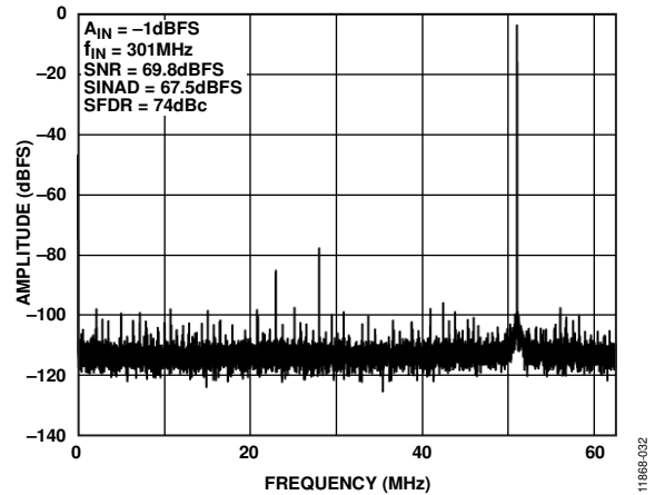
Figure 10. Single-Tone 32k FFT with f_{IN} = 301 MHz , f_{SAMPLE} = 125 MSPS , V_{REF} = 1.4 V
