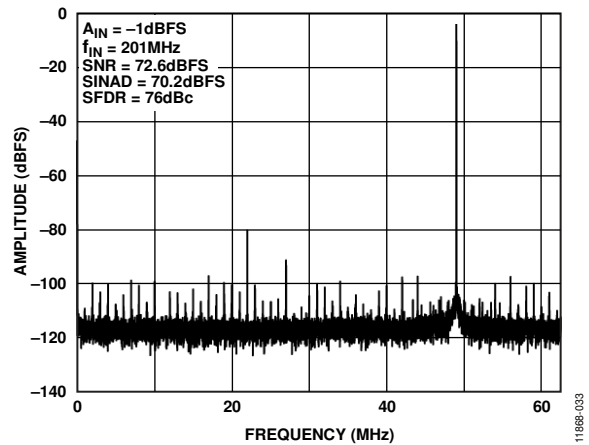
Figure 9. Single-Tone 32k FFT with f_{IN} = 201 MHz , f_{SAMPLE} = 125 MSPS , V_{REF} = 1.4 V
