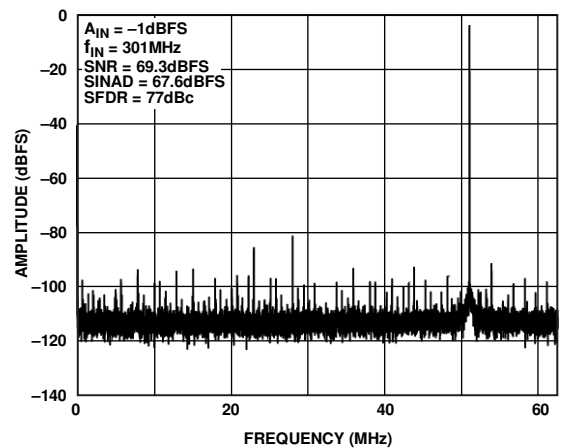
Figure 26. Single-Tone 32k FFT with f_{IN} = 301\text{ MHz} , f_{SAMPLE} = 125\text{ MSPS} , V_{REF} = 1.0\text{ V}
