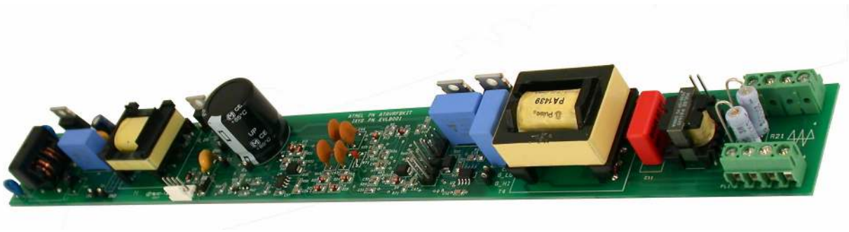
Figure 1-2. Ballast Demonstrator Board
