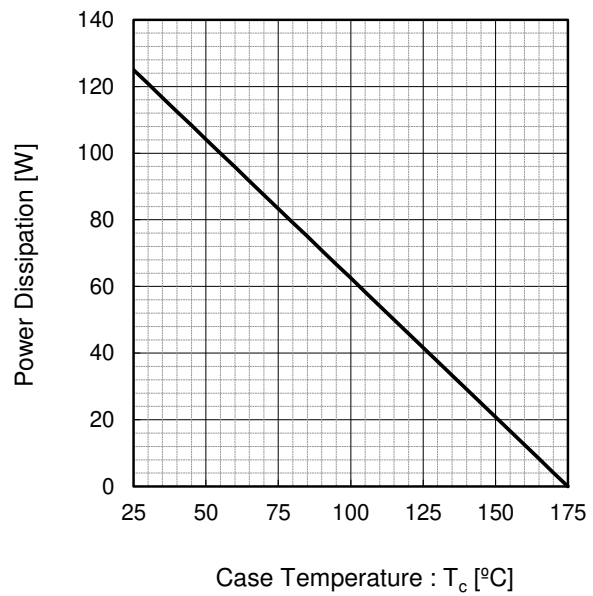
Fig.6 Power Dissipation
