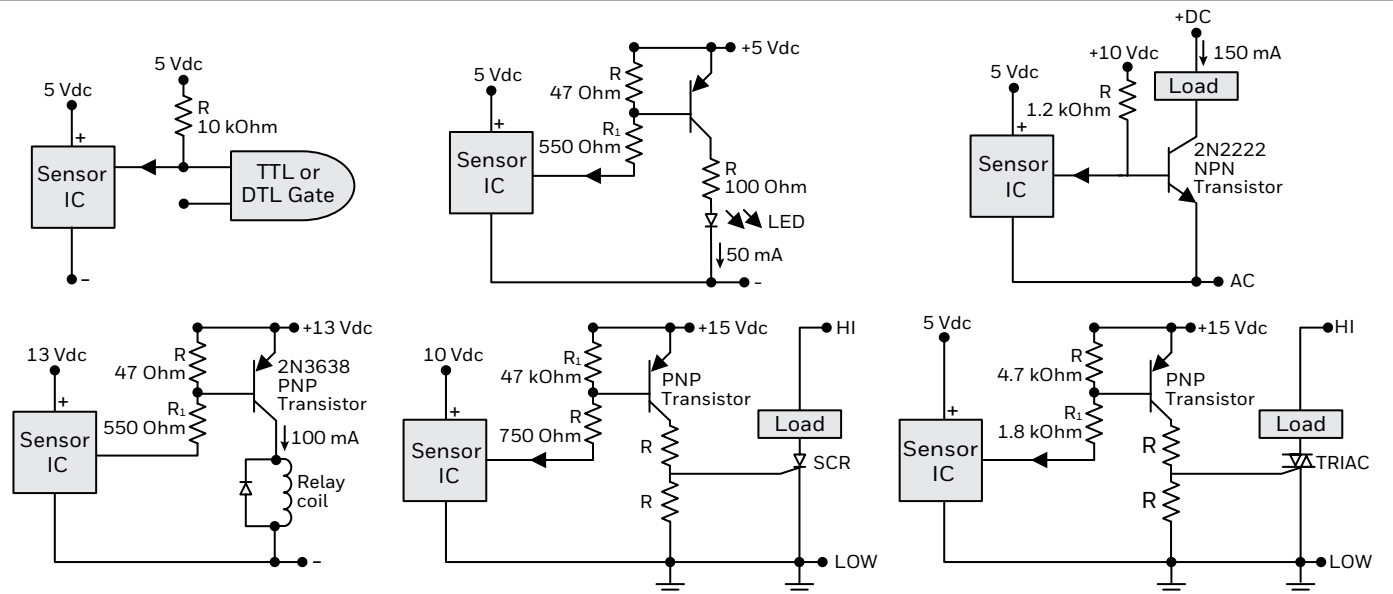
Figure 7. Wiring Diagrams
