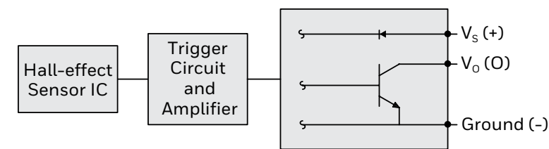
Figure 7. Wiring Diagrams
