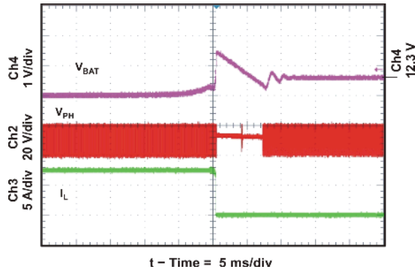
BATTERY REMOVAL
