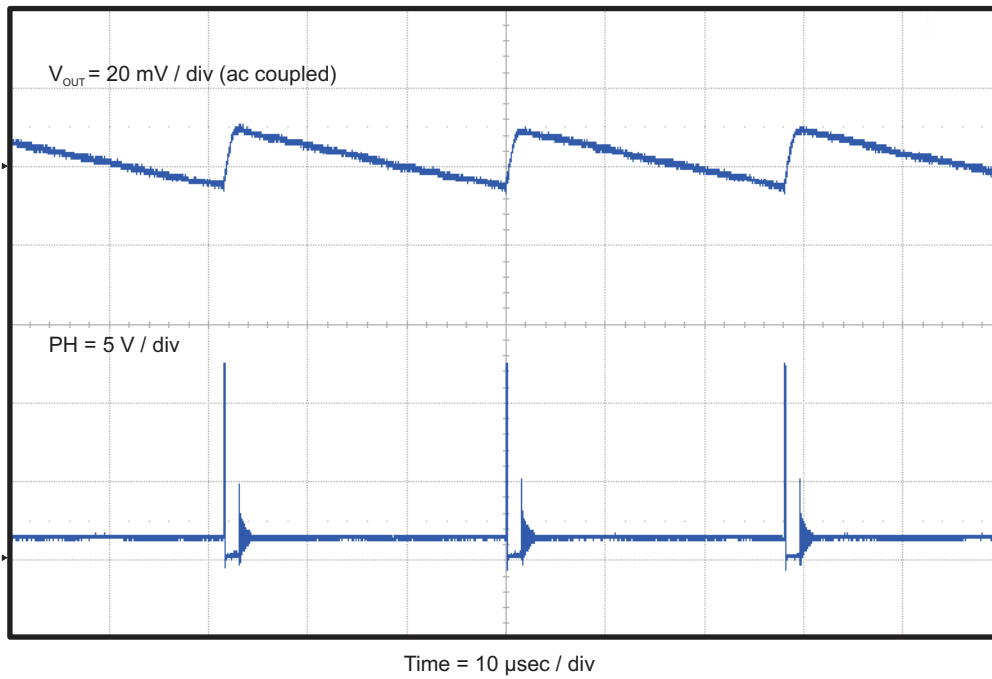
Figure 4-9. TPS54329EEVM-056 Eco-mode Output Voltage Ripple
