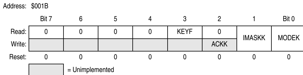
Figure 22-3. Keyboard Status and Control Register (KBSCR)
