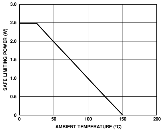
Figure 2. Thermal Derating Curve, Dependence of Safety Limiting Values with Ambient Temperature per DIN V VDE V 0884-10
