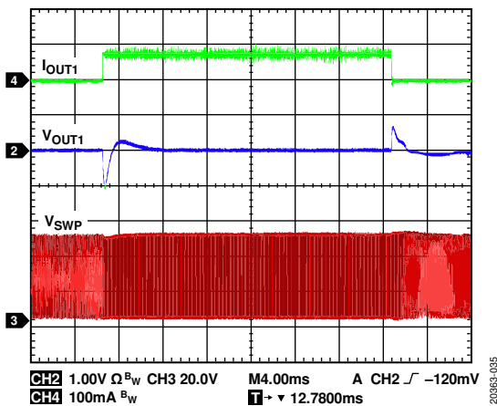
Figure 30. Flyback Regulator Load Transient Response, V_{INP} = 24\text{ V} , V_{OUT1} = 24\text{ V} , I_{OUT1} = 1\text{ mA} to 80\text{ mA} Step, T_A = 25^\circ\text{C}
