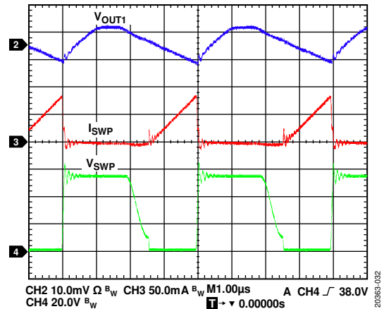
Figure 31. Flyback Regulator Discontinuous Conduction Mode Operation Showing I_{SWP} , Switch Node Voltage, and Output Ripple, T_A = 25^\circ\text{C} , V_{INP} = 24\text{ V} , V_{OUT1} = 24\text{ V} , I_{OUT1} = 20\text{ mA}
