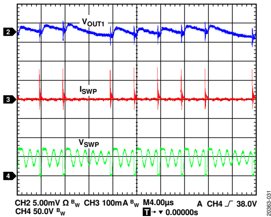
Figure 29. Flyback Regulator Pulse Skipping Operation Showing Inductor Current ( I_{SWP} ), Switch Node Voltage, and Output Ripple, T_A = 25^\circ\text{C} , V_{INP} = 48\text{ V} , V_{OUT1} = 24\text{ V} , I_{OUT1} = 4\text{ mA}
