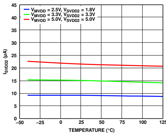
Figure 63. I_{SVDD2} vs. Temperature at Various Supply Voltages, SSS Low, Data Rate = 40 kbps on All GPIO Channels
