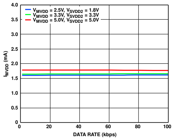
Figure 59. I_{MVDD} vs. Data Rate on All GPIO Channels at Various Supply Voltages, MSS High
