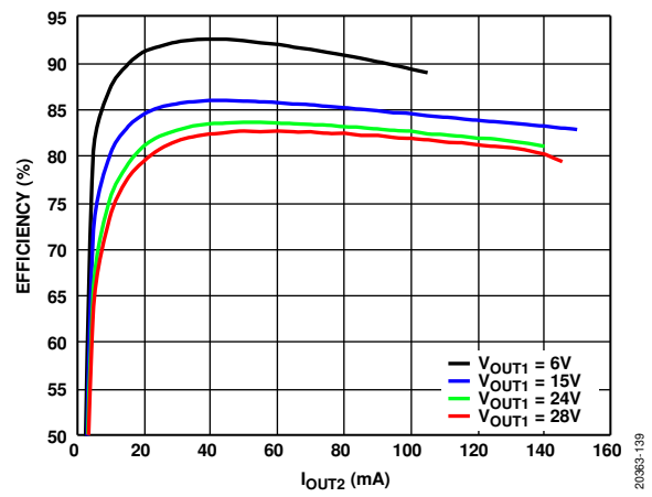
Figure 39. Buck Regulator Efficiency vs. Load Current over Various V_{OUT1} , V_{OUT2} = 5.0\text{ V} , T_A = 25^\circ\text{C}
