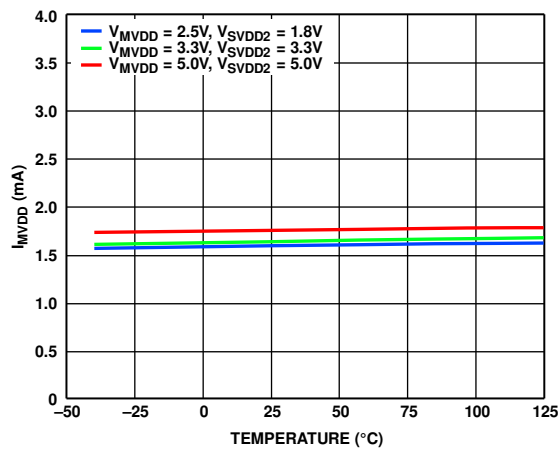
Figure 60. I_{MVDD} Supply Current vs. Temperature at Various Supply Voltages, MSS Low, Data Rate = 40 kbps on All GPIO Channels
