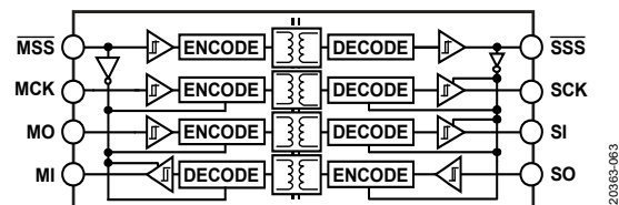
Figure 69. High Speed Data Isolation Channel Gating
