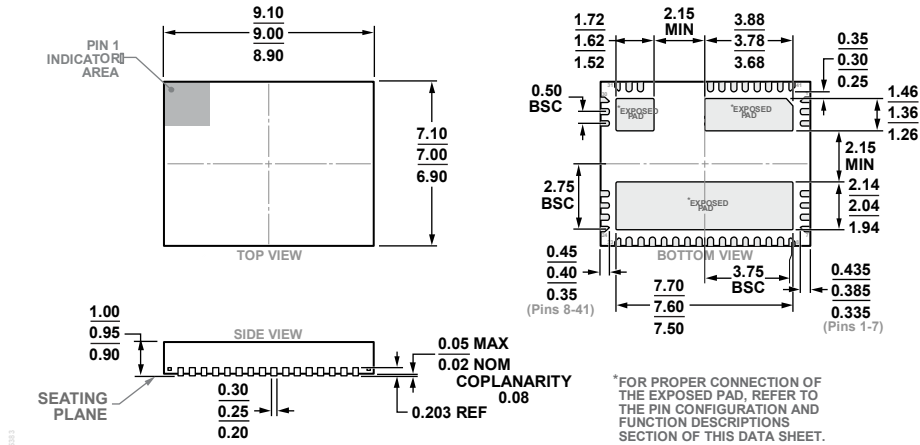
Figure 79. 41-Lead Lead Frame Chip Scale Package [LFCSP] 9 mm × 7 mm Body and 0.95 mm Package Height (CP-41-1) Dimensions shown in millimeters
