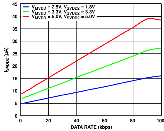
Figure 62. SVDD2 Supply Current ( I_{SVDD2} ) vs. Data Rate on All GPIO Channels at Various Supply Voltages, MSS High
