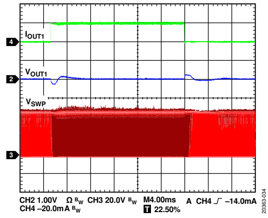
Figure 33. Flyback Regulator Load Transient Response, V_{INP} = 24\text{ V} , V_{OUT1} = 24\text{ V} , I_{OUT1} = 1\text{ mA} to 20\text{ mA} Step, T_A = 25^\circ\text{C}
