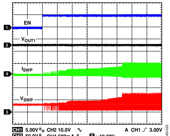
Figure 32. Flyback Regulator Short-Circuit Current Limit During Startup, V_{INP} = 24\text{ V} , V_{OUT1} = \text{SGND2} , T_A = 25^\circ\text{C}
