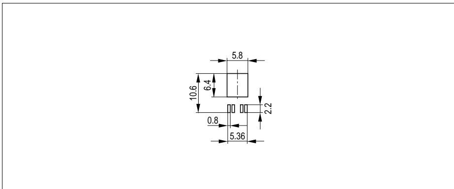
Figure 6 Foot Print for P-TO-252-5-1 and P-TO-252-5-11 (Plastic Transistor Single Outline)
