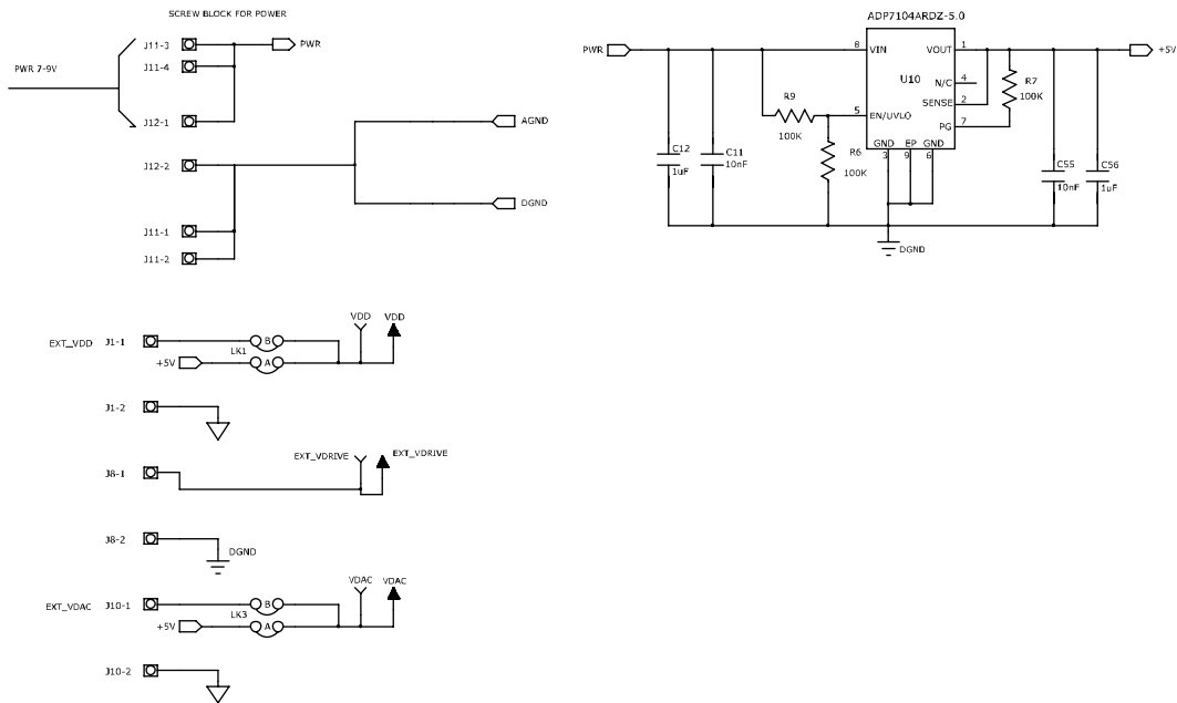
Figure 9. Schematic of AD7294-2 Power Supply Circuitry
