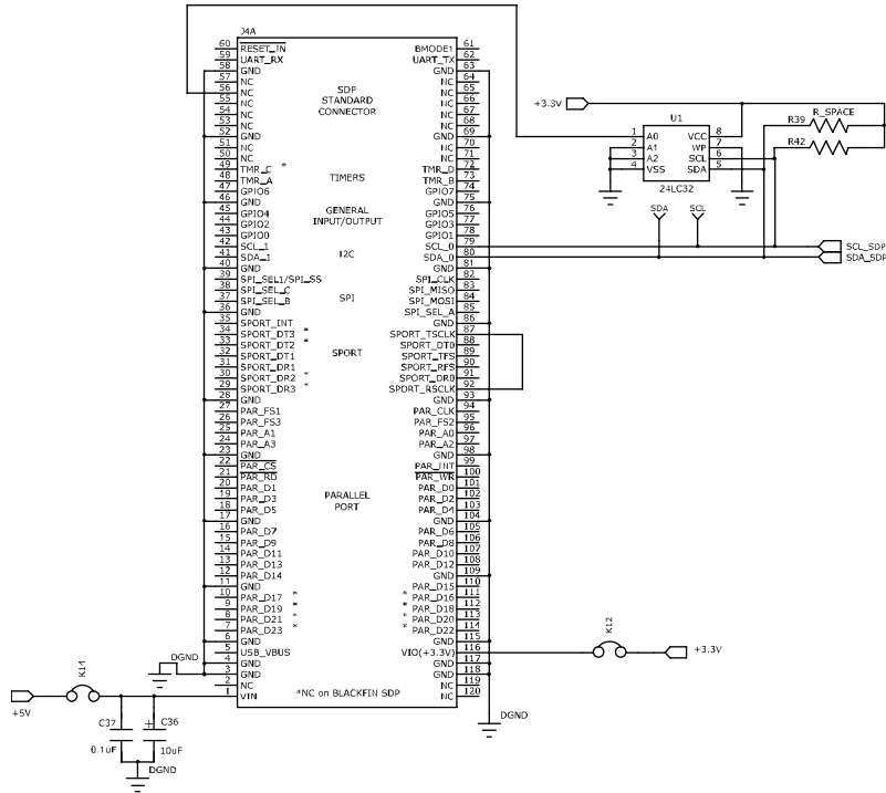
Figure 8. Schematic of SDP Circuitry
