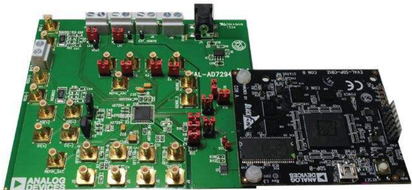
Figure 1. Universal Evaluation Board Connected to the SDP-B Board
