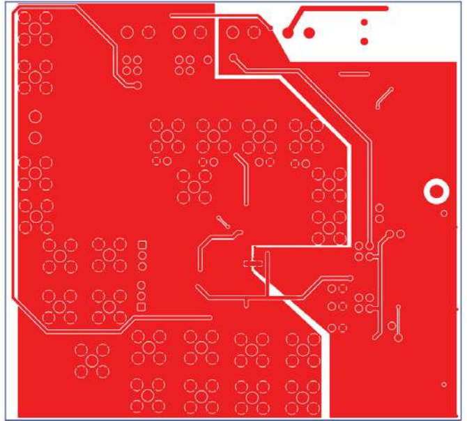
Figure 12. Solder Side PCB Drawing
