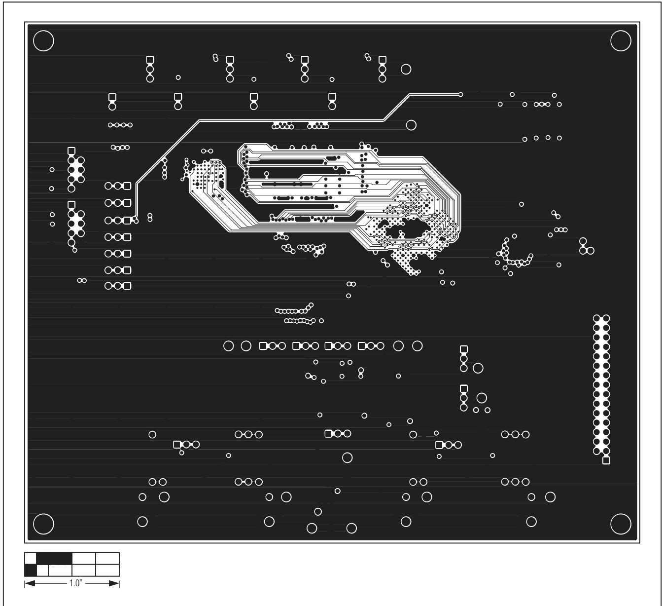
Figure 13. MAX1103 EV Kit PCB Layout—Layer 6
