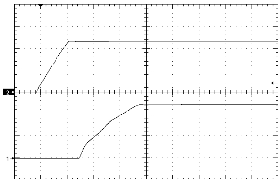
Figure 10. Startup Waveform via Input Voltage, time scale 4mS/div. Vin=Vin_nom, Iout=full load Cout=0uF, Ch1=Vout (2V/div), Ch2=Vin (20V/div)
