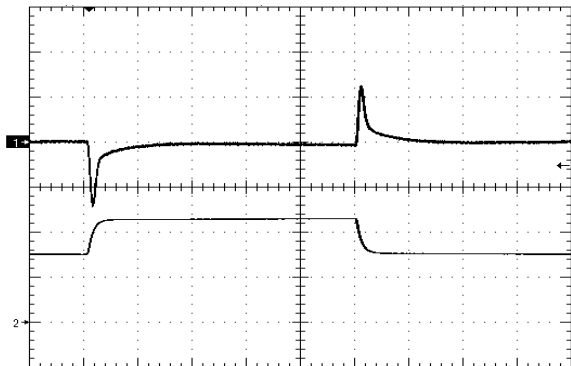
Figure 12. Load Transient Response (100mV/div), di/dt=0.1A/uS, 50%-75%-50% of full Iout, Cout=Fig16 time scale: 200uS/div. Ch1=Vout, Ch2=Iout (1A/div)
