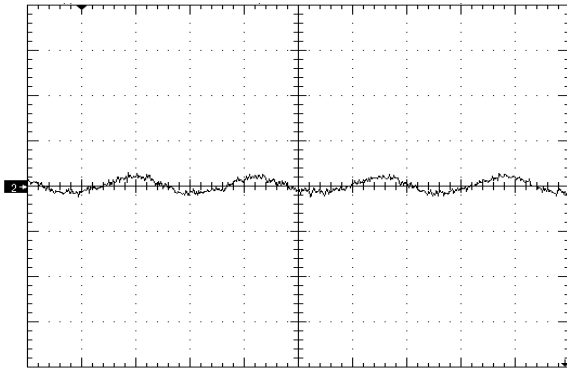
Figure 7. Input Reflected Ripple Current (10mA/div), time scale – 1uS/div. Vin=Vin_nom, full load (see Fig 15)
