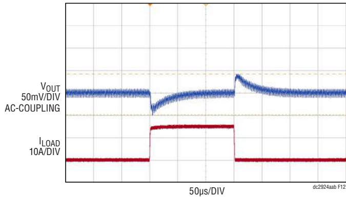
CIRCUIT CONFIGURATION: 4-PHASE 4 OUTPUTS f_{SW} = 350\text{kHz} V_{OUT} = 1\text{V} I_{LOAD-STEP} = 0\text{A TO } 15\text{A AT } diL/dt = 15\text{A}/\mu\text{s} V_{OUT(P-P)} = 91\text{mV} OUTPUT VOLTAGE WAS MEASURED AT V_{OUT0} BNC
