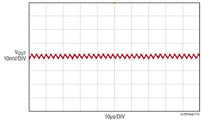
CIRCUIT CONFIGURATION: 4-PHASE SINGLE OUTPUT f_{SW} = 350\text{kHz} V_{OUT} = 1\text{V} I_{LOAD} = 120\text{A} V_{OUT(P-P)} = 4.7\text{mV} OUTPUT RIPPLE VOLTAGE WAS MEASURED ACROSS C_{OUT29} 1x SCOPE PROBE AND PROBE JACK USED AC-COUPLING, 20MHz BWL
