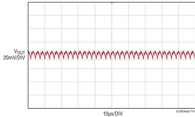
CIRCUIT CONFIGURATION: 4-PHASE 4 OUTPUTS f_{SW} = 350\text{kHz} V_{OUT} = 1\text{V} I_{LOAD} = 30\text{A} V_{OUT(P-P)} = 13.1\text{mV} OUTPUT RIPPLE VOLTAGE WAS MEASURED AT V_{OUT0} BNC AC-COUPLING, 20MHz BWL
