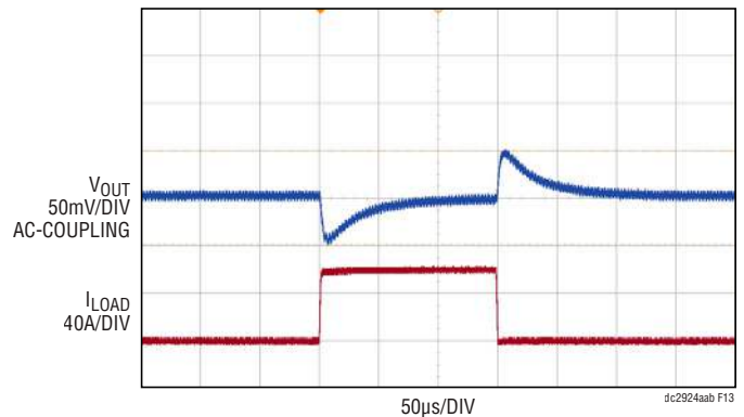
CIRCUIT CONFIGURATION: 4-PHASE SINGLE OUTPUT f_{SW} = 350\text{kHz} V_{OUT} = 1\text{V} I_{LOAD-STEP} = 0\text{A TO } 60\text{A AT } diL/dt = 60\text{A}/\mu\text{s} V_{OUT(P-P)} = 98\text{mV} OUTPUT VOLTAGE WAS MEASURED ACROSS C_{OUT29}
