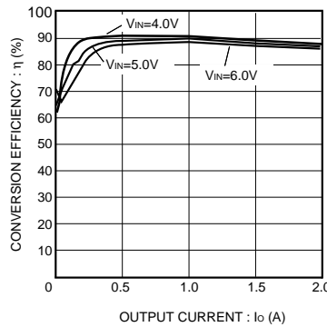
Fig.7 Conversion efficiency
