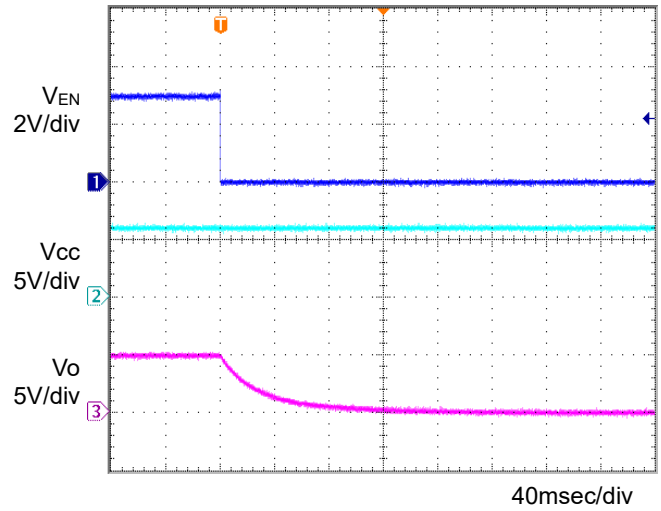
Figure 20. OFF sequence 2 Co=1μF, Ta=105°C
