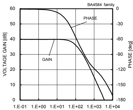
Fig. 154 Voltage Gain - Frequency (VCC/VEE=+15[V]/-15[V], Av=40[dB], RL=2[kΩ], Ta=25[°C])
