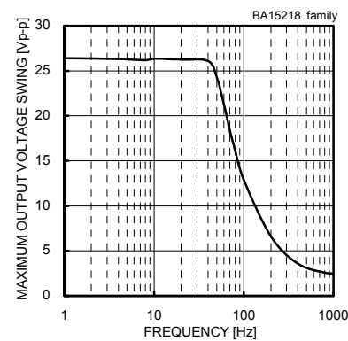
Fig. 219 Maximum Output Voltage Swing - Frequency (VCC/VEE=+15[V]/-15[V], RL=2[kΩ], Ta=25[°C])
