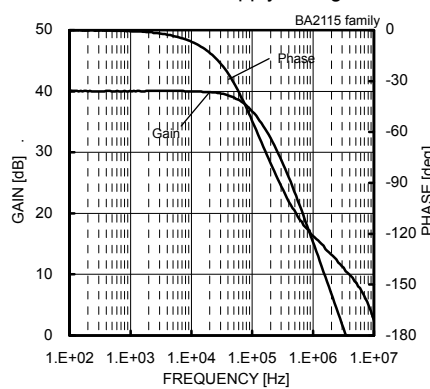
Fig. 310 Voltage Gain - Frequency (VCC/VEE=2.5[V]/-2.5[V], Av=40[dB], RL=10[kΩ])
