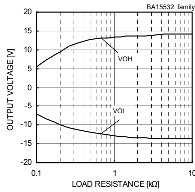
Fig. 247 Maximum Output Voltage - Load Resistance (VCC/VEE=+15[V]/-15[V], Ta=25[°C])
