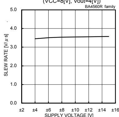
Fig. 84 Slew Rate - Supply Voltage (CL=100[pF], RL=2[kΩ], Ta=25[°C])
