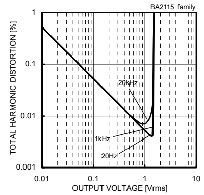
Fig. 308 Total Harmonic Distortion - Output Voltage (VCC/VEE=2.5[V]/-2.5[V], RL=3[kΩ] 80[kHz]-LPF, Ta=25[°C])
