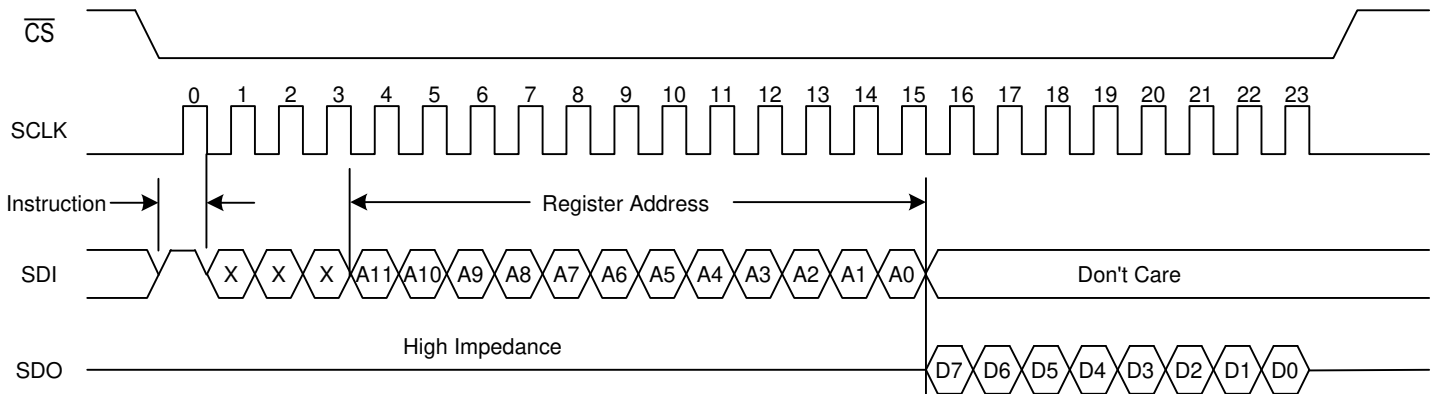
Figure-21 Read Operation In SPI Mode
