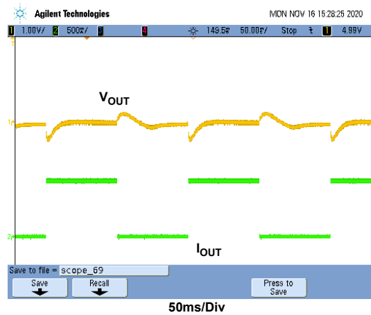
Figure 19. Dynamic Load (0% ~ 100%)
