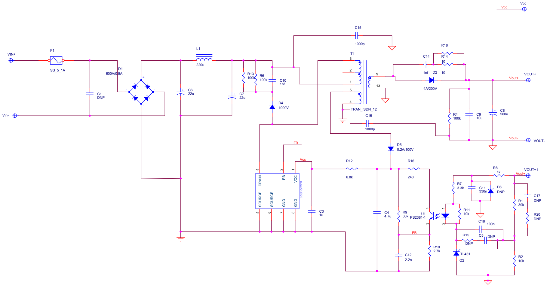
Figure 6. Schematic
