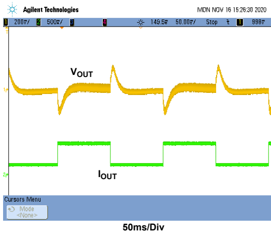
Figure 18. Dynamic Load (25% ~ 75%)
