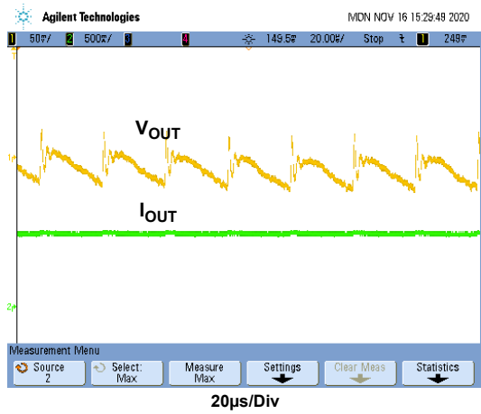
Figure 17. Output Ripple at 1A Load
