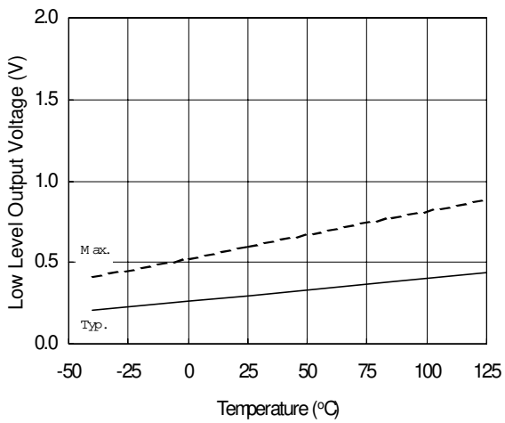
Figure 11A. Low Level Output Voltage vs. Temperature
