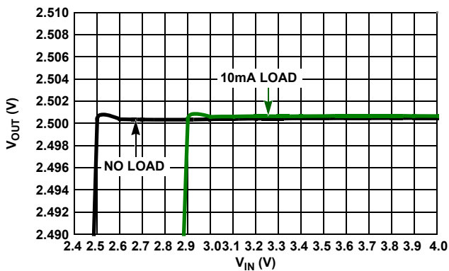
FIGURE 12. DROPOUT
