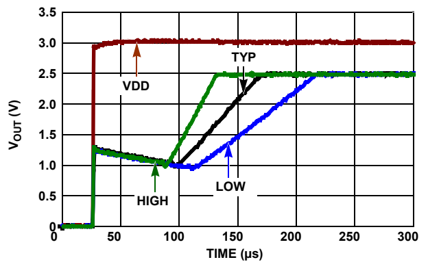
FIGURE 13. TURN-ON TIME
