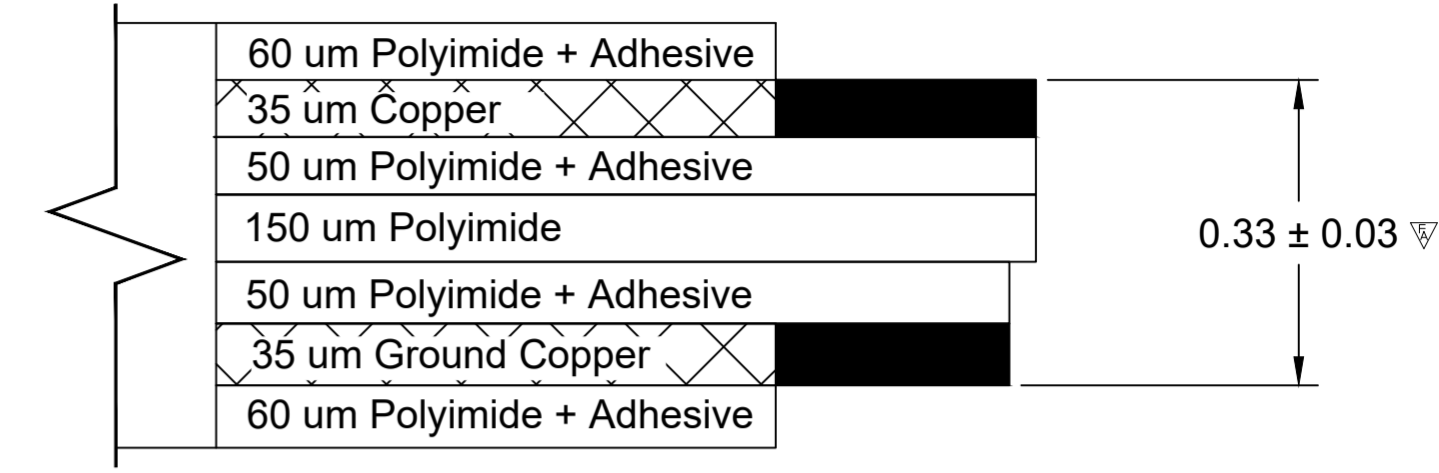
TAIL CROSS-SECTION
