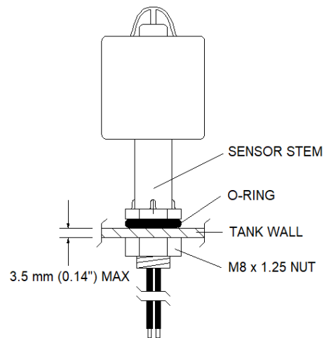
O-ring Placement
