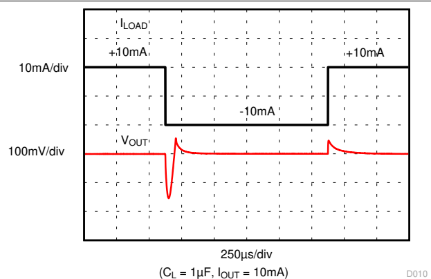
Figure 7-12. Load Transient
