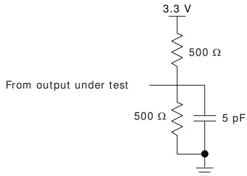
Figure 22 • Test Circuit for TDO Disable Time
