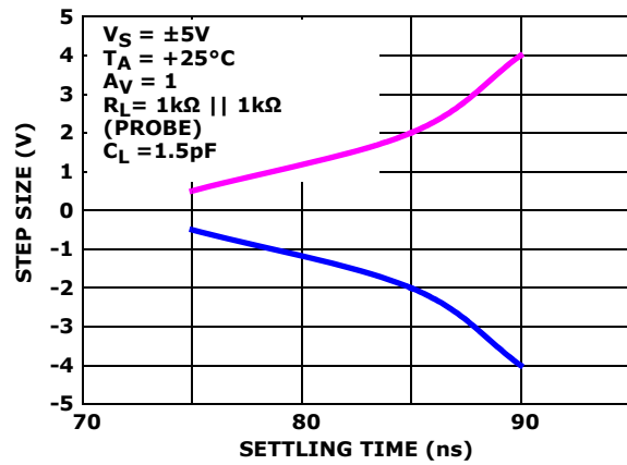
FIGURE 28. STEP SIZE vs SETTLING TIME
