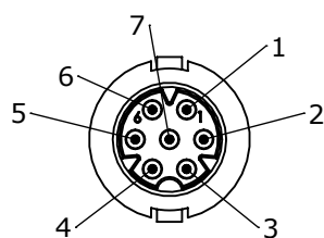
FACE VIEW 16980-7PG-5XX 7 POSITION A-KEY
