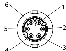
FACE VIEW 16980-6PG-5XX 6 POSITION B-KEY
