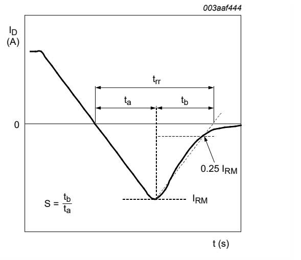
Fig. 17. Reverse recovery timing definition
