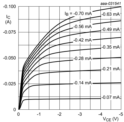
Fig. 10. NHUMB11: Collector current as a function of collector-emitter voltage; typical values
