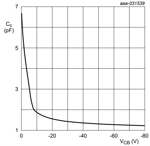
Fig. 8. NHUMB11: Collector capacitance as a function of collector-base voltage; typical values
