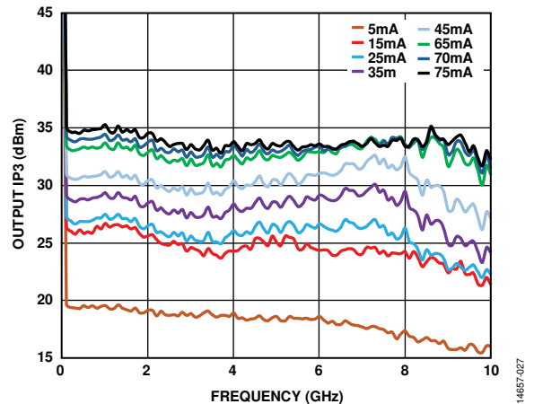
Figure 28. Output IP_3 vs. Frequency for Various Supply Currents ( I_{DQ} ), P_{OUT}/Tone = 5 dBm , V_{DD} = 5 V
