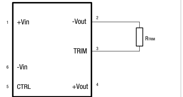
Figure 2. Trim connections to increase the output voltage
