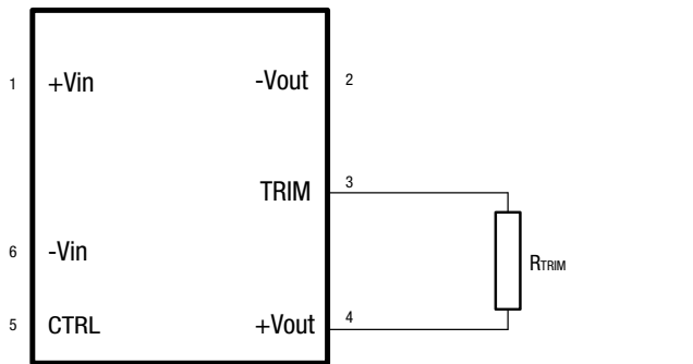
Figure 1. Trim connections to decrease the output voltage
