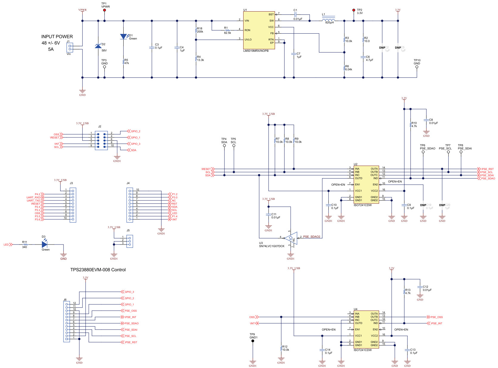
Figure 12. BOOST-PSEMTHR-007 (Motherboard) Schematic: Control
