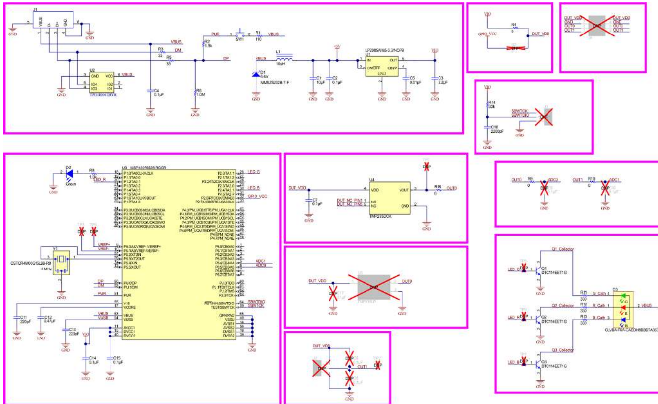
Figure 18. EVM Schematic
