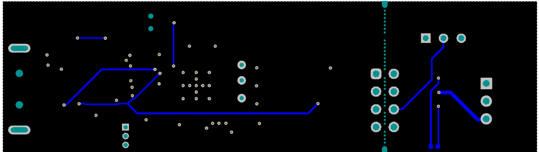
Figure 23. Bottom Signal Layer
