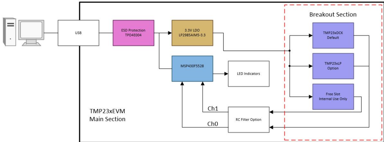
Figure 4. EVM Block Diagram
