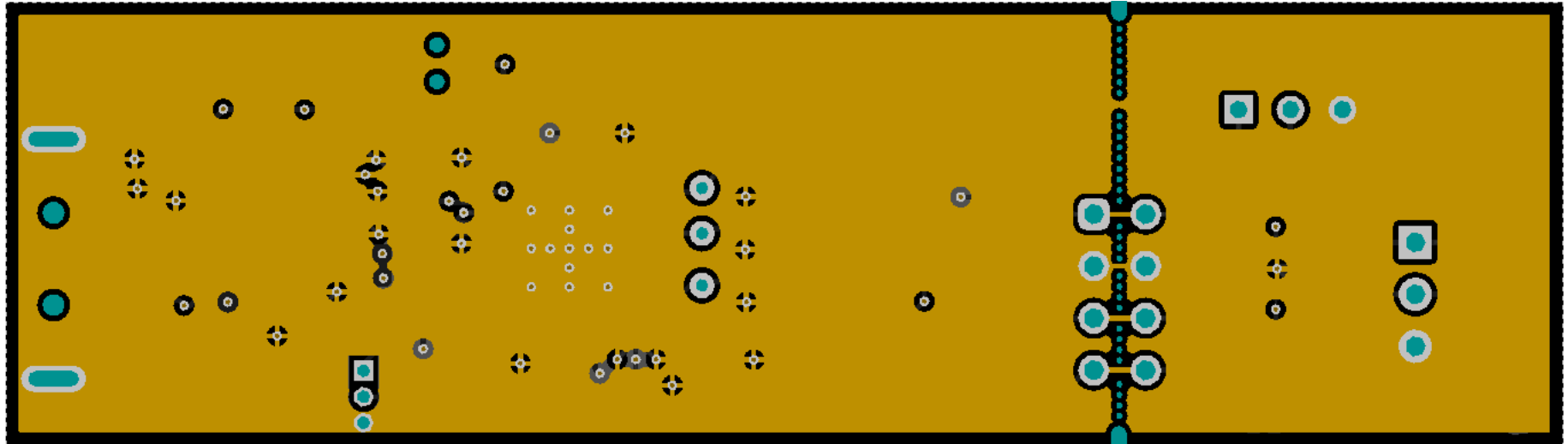
Figure 21. Ground Layer
