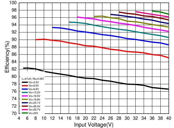
Efficiency vs. Input Voltage (MSOP-8EP, R_s=0.067\Omega , L=47\mu\text{H} )
