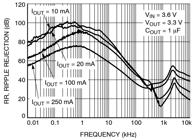
Figure 23. Power Supply Rejection Ratio, V_{OUT} = 3.3 \text{ V}
