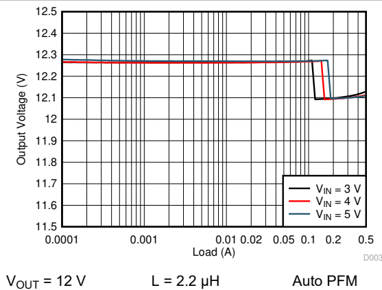
Figure 6-3. Load Regulation
