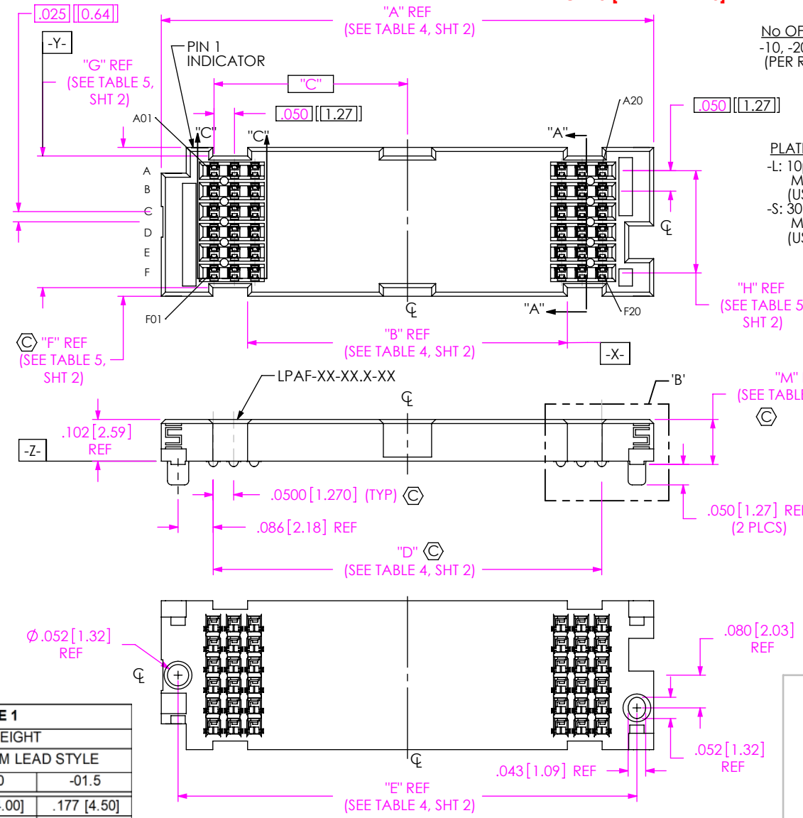
FIG 1 LPAF-20-03.0-X-06-X-K-XR SHOWN (SOME FEATURES REMOVED FOR CLARITY)
