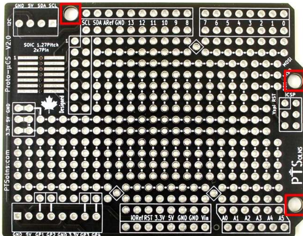
Figure 8: Mounting holes.
