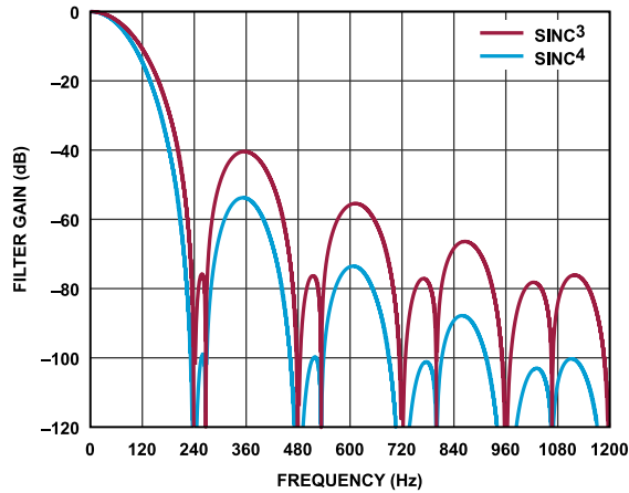
Figure 85. Sinc 3 and Sinc 4 Filter Response (FS = 0d10)
