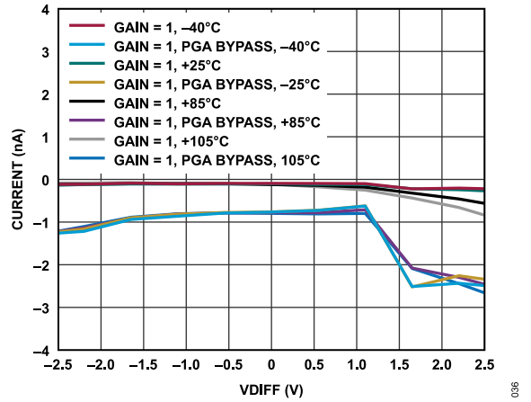
Figure 36. Absolute AINM Current vs. VDIFF for Various Temperatures (Gain = 1, VCM = AV DD /2)
