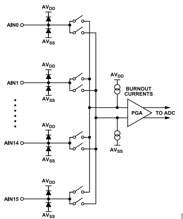
Figure 70. Analog Input Multiplexer Circuit
