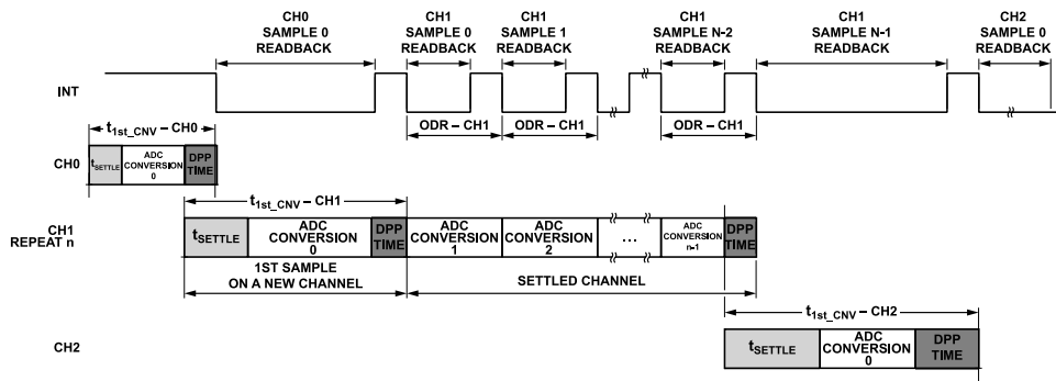
Figure 94. Example of Smart Sequencing
