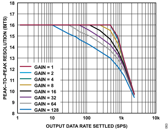
Figure 63. Peak-to-Peak Resolution vs. Output Data Rate (Settled) for Various Gains (Sinc³ Filter)
