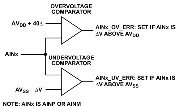
Figure 98. Analog Input Overvoltage/Undervoltage Monitors
