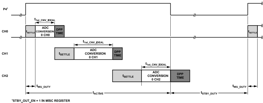
Figure 95. Example of Autonomous Duty Cycling Mode
