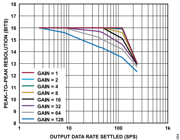
Figure 64. Peak-to-Peak Resolution vs. Output Data Rate (Settled) for Various Gains (Sinc³ + Sinc¹ Filter)
