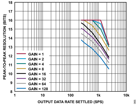
Figure 65. Peak-to-Peak Resolution vs. Output Data Rate (Settled) for Various Gains (Sinc⁴ Filter)
