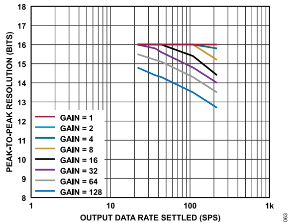
Figure 66. Peak-to-Peak Resolution vs. Output Data Rate (Settled) for Various Gains (Sinc⁴ + Sinc¹ Filter)
