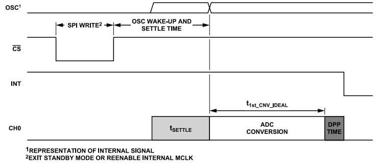
Figure 96. Out of Standby Mode Diagram
