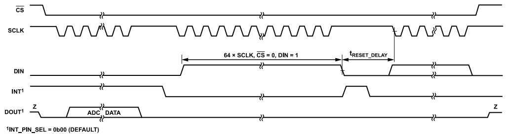
Figure 75. Software Reset Timing Diagram
