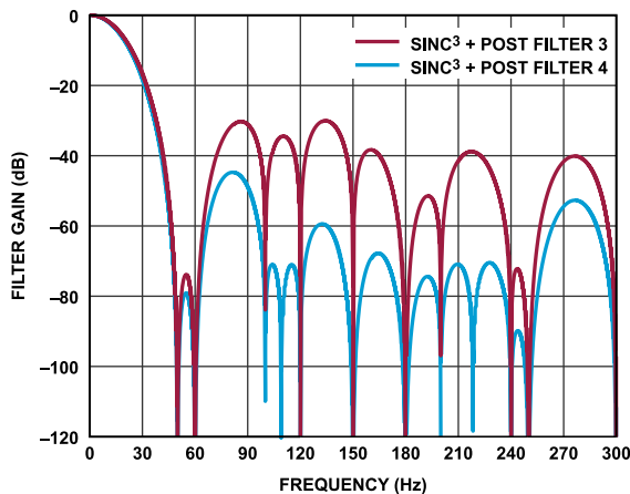
Figure 87. Post Filter 3 and Post Filter 4 Response
