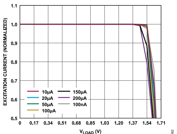
Figure 62. Output Compliance for Various IEXC Sources ( AV_{DD} = 1.71\text{ V} )
