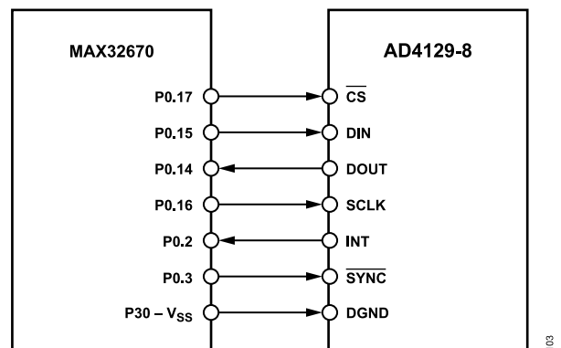
Figure 107. Example of MAX32670 \mu C SPI Connection to AD4129-8
