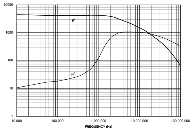
44 MATERIAL PERMABILITY VS FREQUENCY
