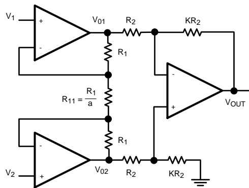
Figure 5. Instrumentation Amplifier
