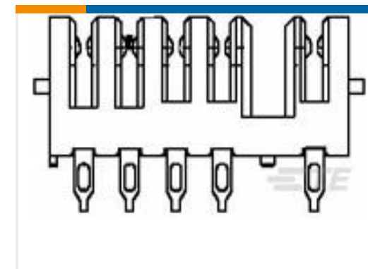
TE Part #1565986-1 REC ASSY,2.5 SLIM BATTERY CONN
