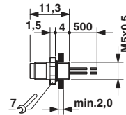
Dimensioned drawing
