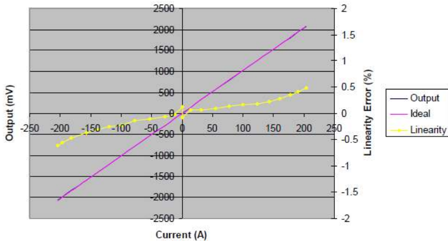
RAZFL-204CMCG TYPICAL PERFORMANCE
