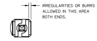
DETAIL Z SCALE 5:1
