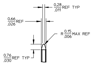
DETAIL Y SCALE 5:1 SEE NOTE 10
